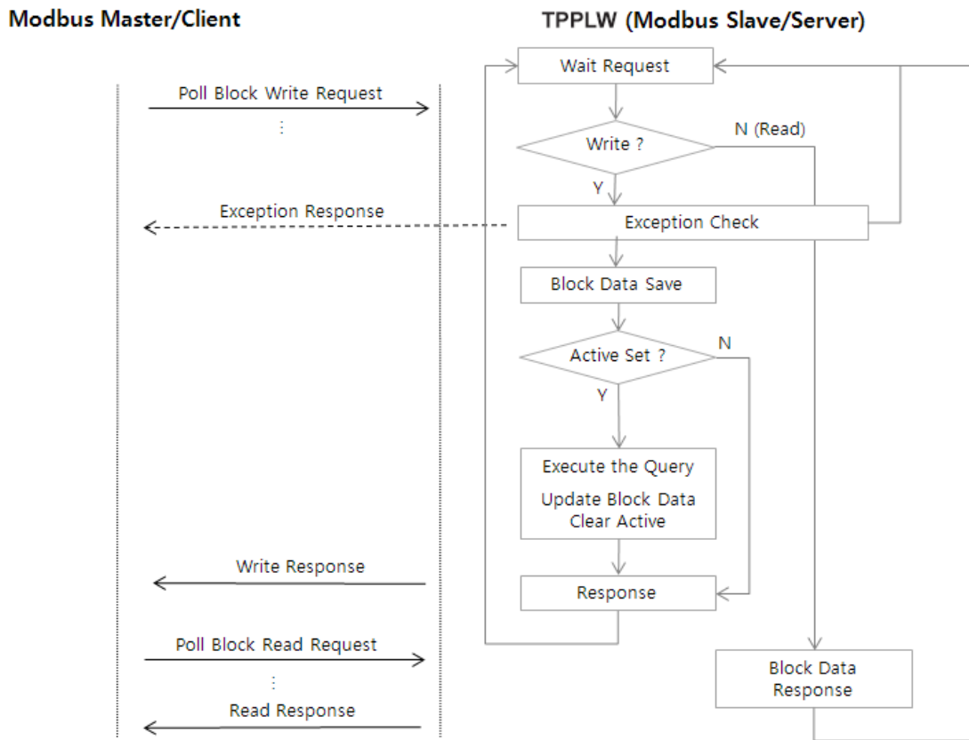
Figure 7. Modbus Query Poll Register processing procedure
