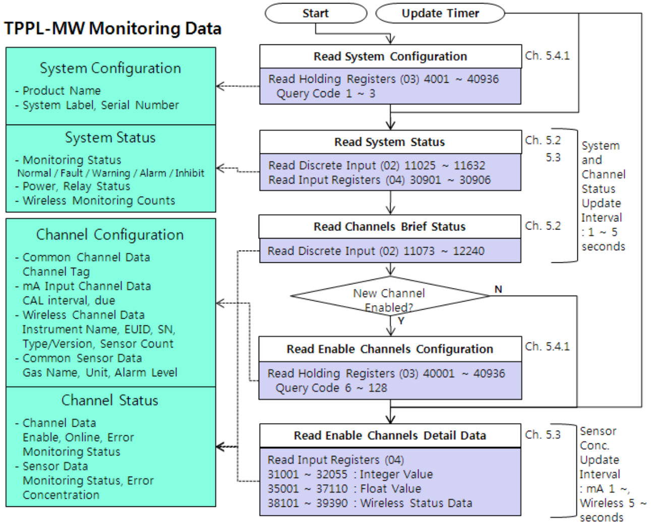
Figure 6. Modbus Register Outline
