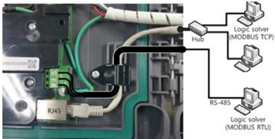
Figure 4. TPPLW Modbus TCP / RTU Client Connections
